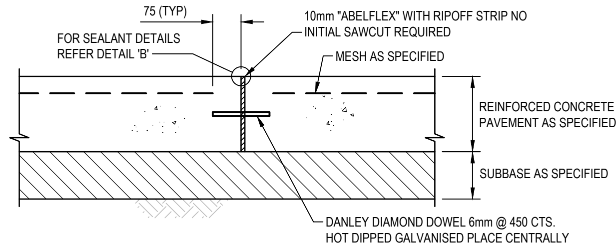
EXPANSION JOINT (EJ) ALSO TRANSVERSE STOP WORK JOINT SCALE 1:10
