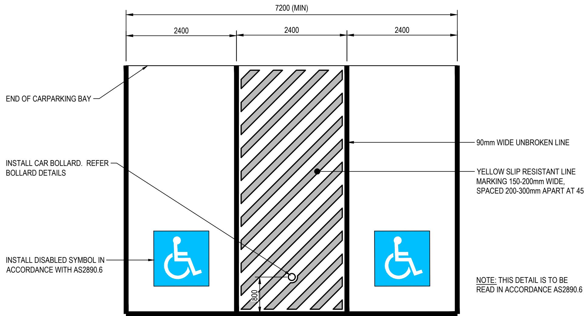
TYPICAL PWD AND SHARED ZONE SCALE 1:50
