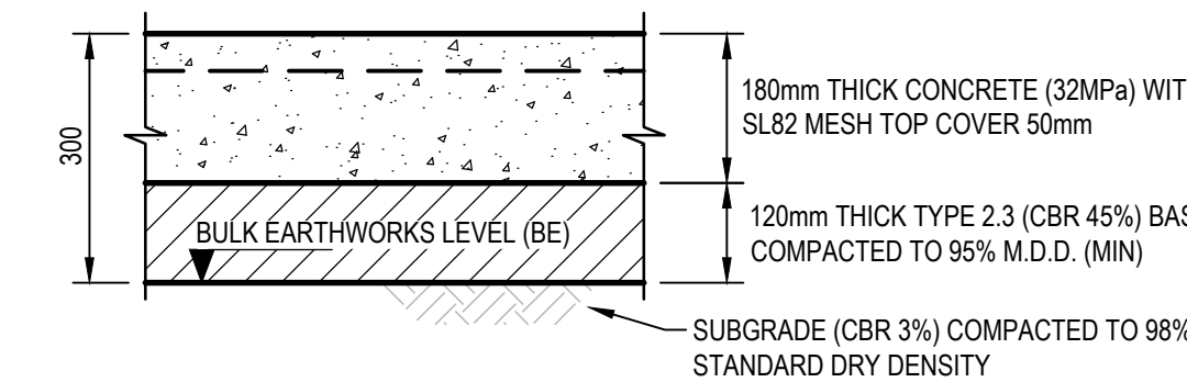
PAVEMENT TYPE 3 HEAVY DUTY CONCRETE PAVEMENT SCALE 1:10
