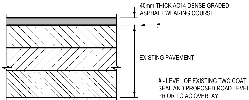
PAVEMENT TYPE 5 AC OVERLAY EXISTING PAVEMENT SCALE 1:10
