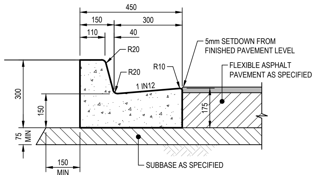
BARRIER KERB AND CHANNEL (BKC) SCALE 1:10
