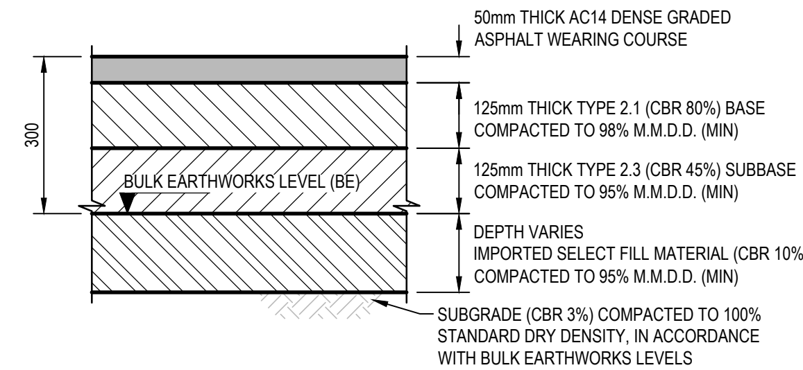
PAVEMENT TYPE 2 HEAVY DUTY ASPHALT FLEXIBLE PAVEMENT SCALE 1:10
