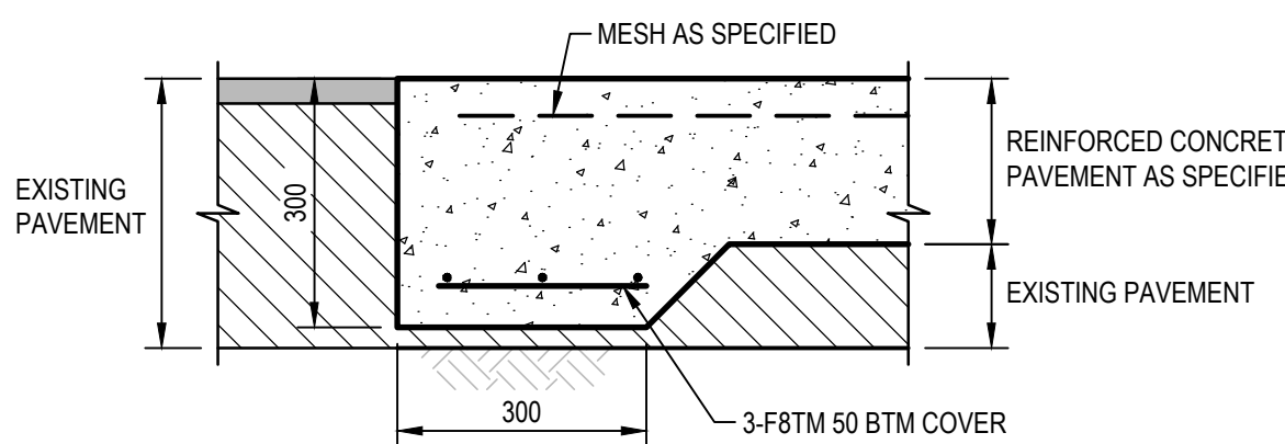
CONCRETE EDGE THICKENING (ET) SCALE 1:10
