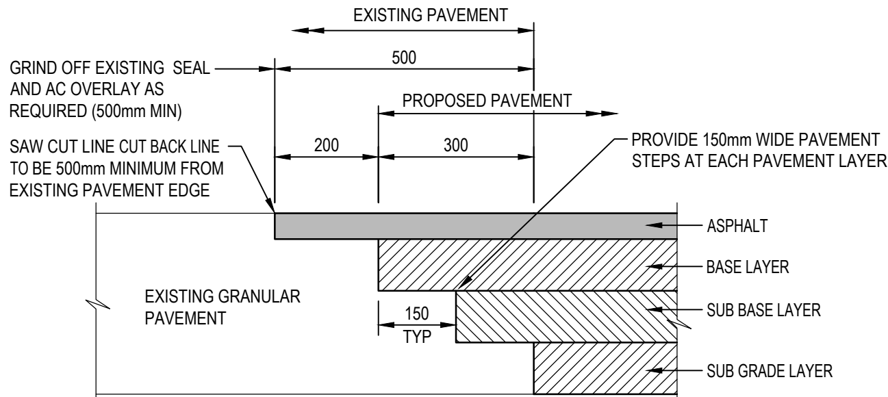
GRANULAR PAVEMENT JOINT DETAIL SCALE 1:10
