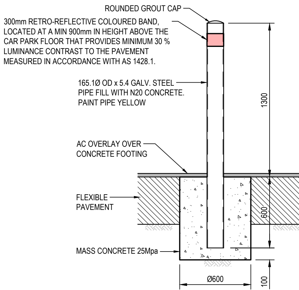
BOLLARD DETAIL CAR BOLLARD IN FLEXIBLE PAVEMENT SCALE 1:20
