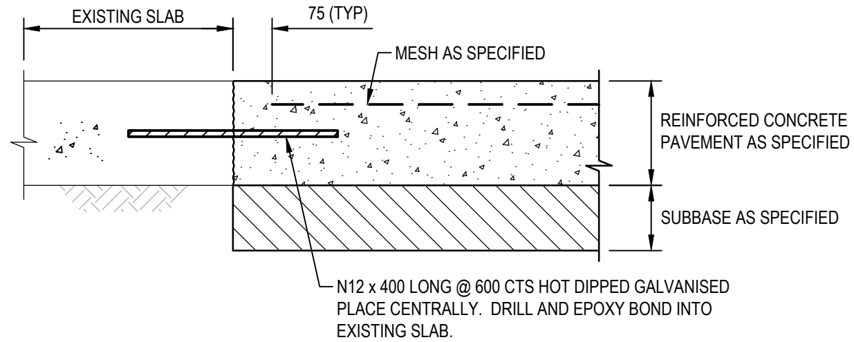
EXPANSION JOINT ABUTTING EXISTING SLAB (EJE) SCALE 1:10
