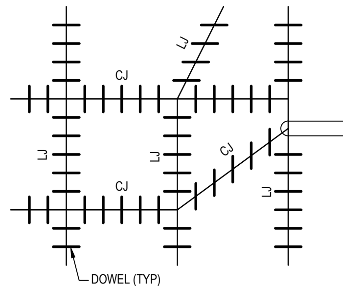
DOWEL ORIENTATIONS NTS
