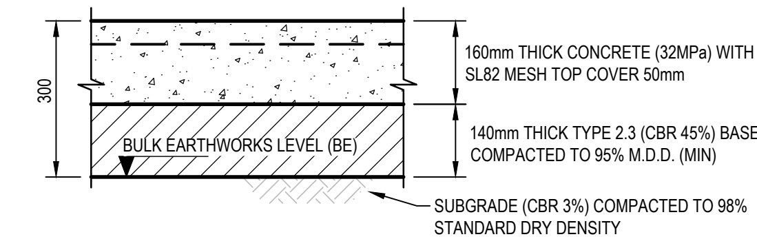
PAVEMENT TYPE 4 LIGHT DUTY CONCRETE PAVEMENT SCALE 1:10
