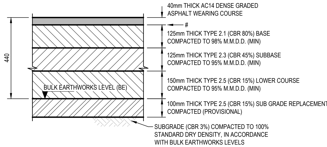
PAVEMENT TYPE 1 LIGHT DUTY ASPHALT FLEXIBLE PAVEMENT SCALE 1:10
