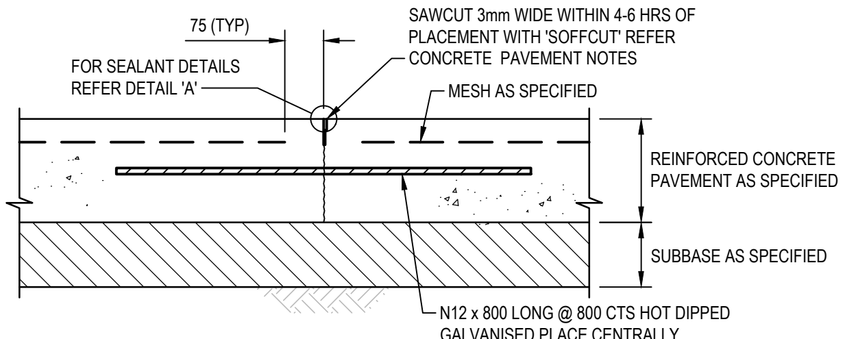
LONGITUDINAL CONTRACTION JOINT (LJ) (POUR OVER) SCALE 1:10
